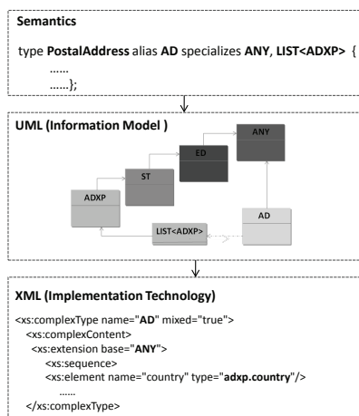
Figure 2.2: HL7 Version 3: Semantics to Implementation Technology
