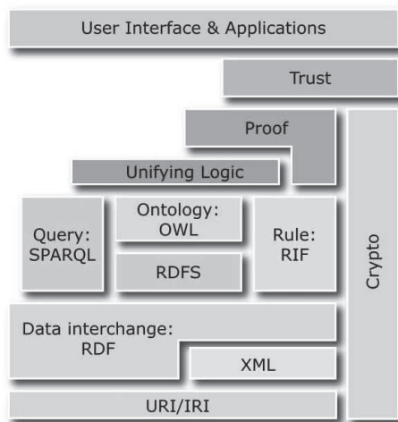
Figure 2.6: The Semantic Web Layer Cake
